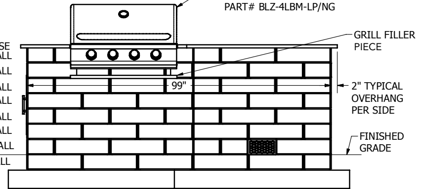
FRONT ELEVATION VIEW
