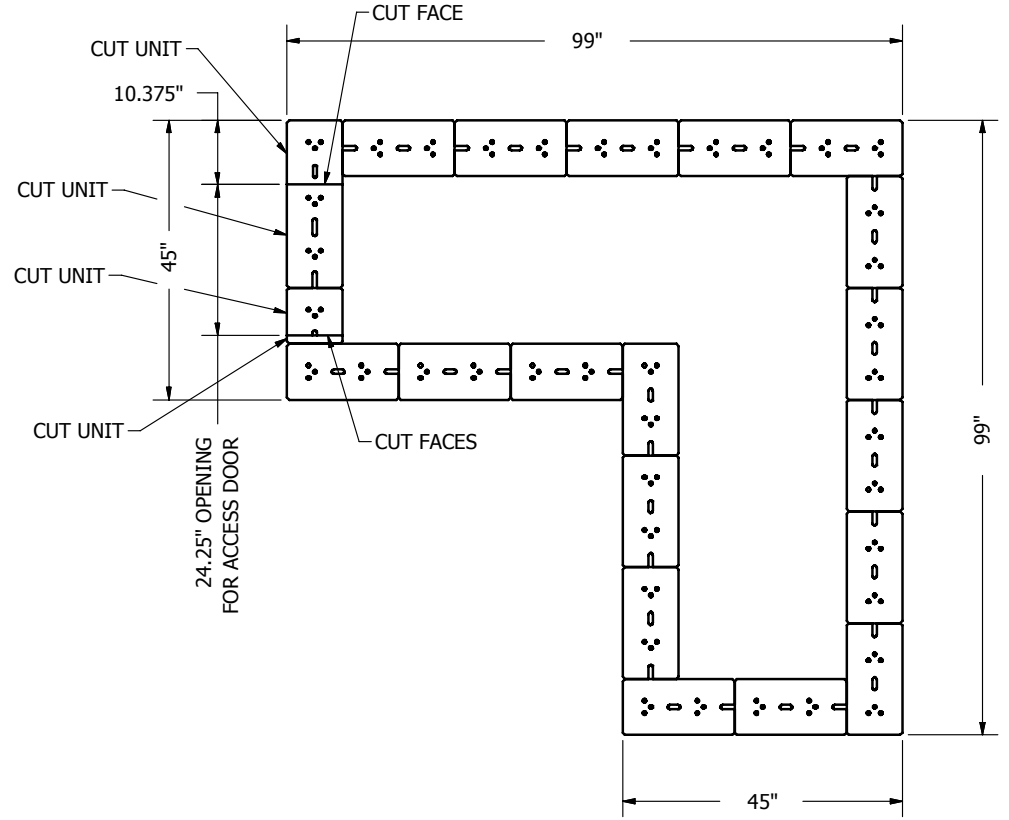
PLAN VIEW
