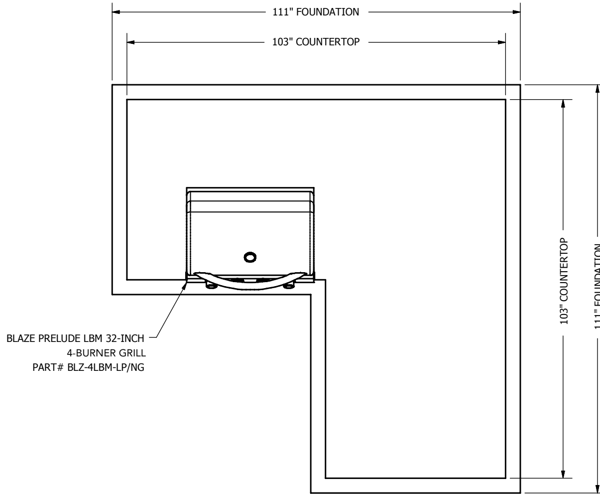
PLAN VIEW
