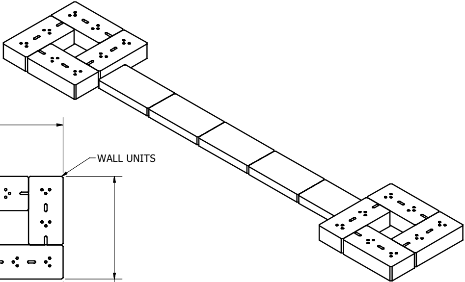
ISOMETRIC VIEW
