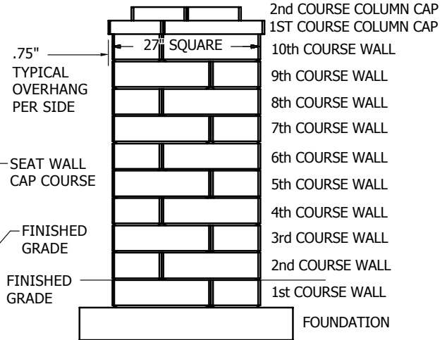
SIDE ELEVATION VIEW
