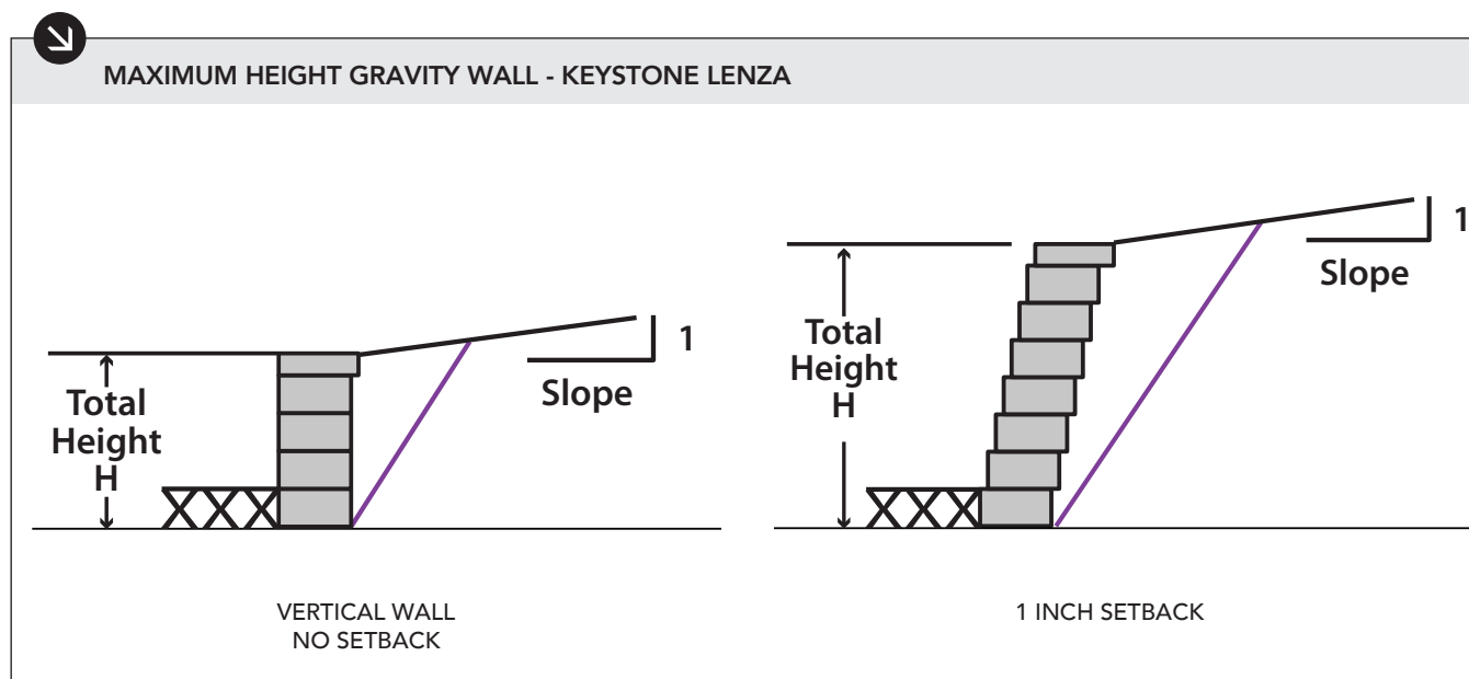
GRAVITY CHART: LENZA (UNIT HEIGHT = 5" AND CAP HEIGHT = 2.5") VERTICAL
