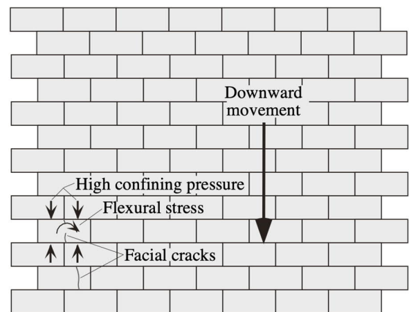
Tall Wall Settlement
