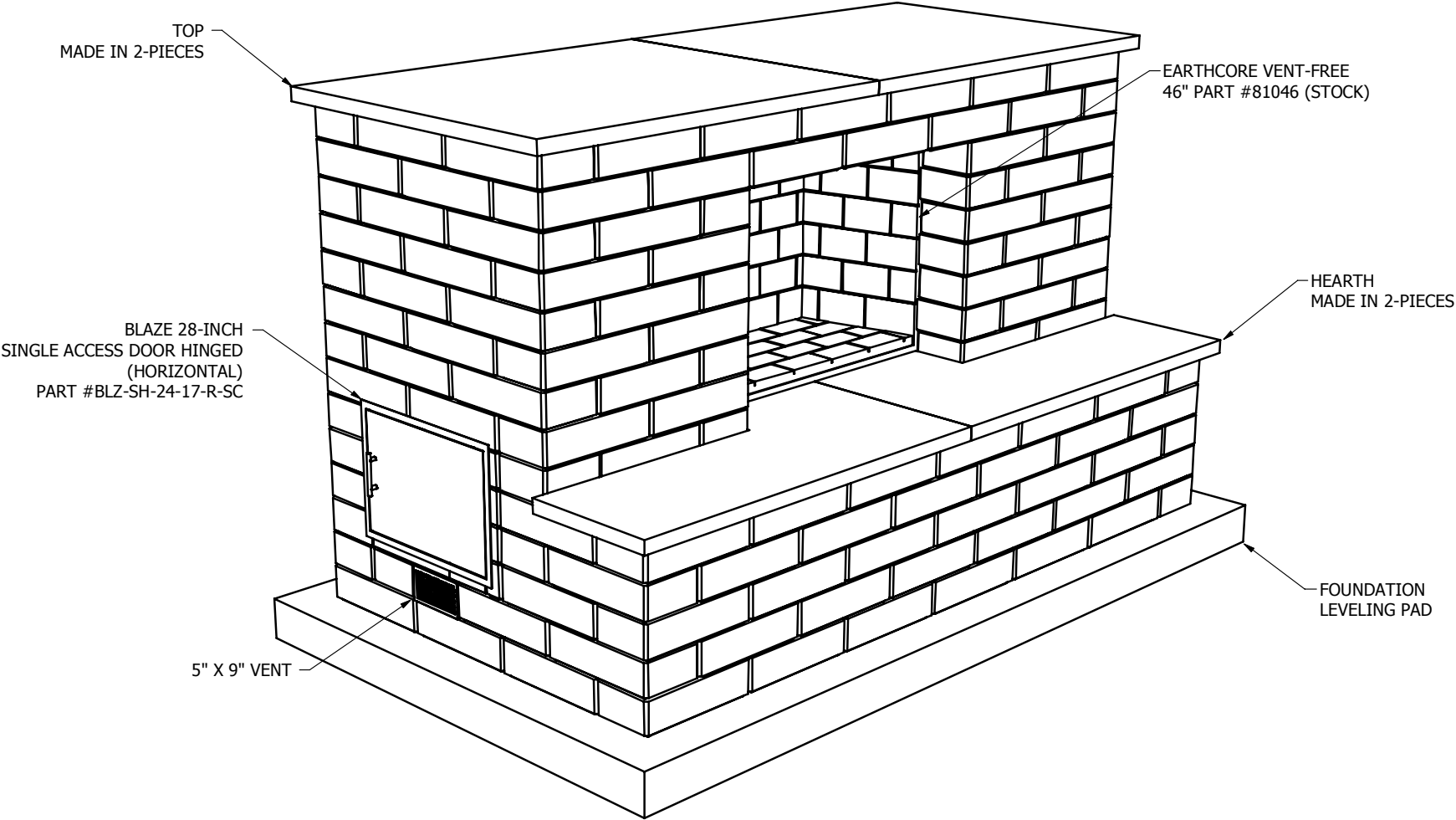
ISOMETRIC VIEW
