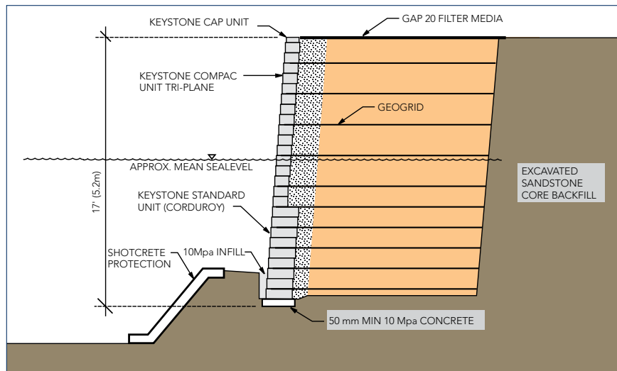
Typical canal wall section.
