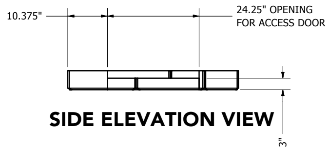
LENZA - 45 x 63 GRILL TOP - RIGHT DOOR CUT DESIGN - 3rd COURSE
