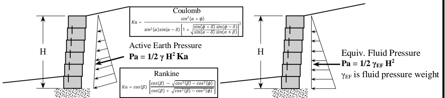
Active Earth Pressure
