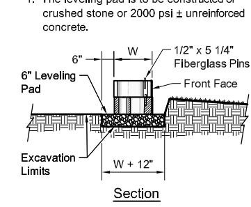
Leveling Pad Detail
