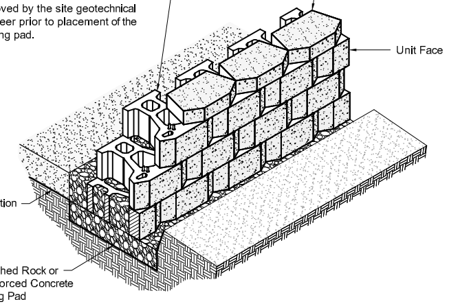
Standard III Unit/Base Pad Isometric Section View * Dimensions & Weight May Vary by Region
