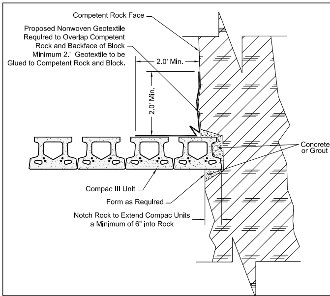
Joint detail at competent rock.
