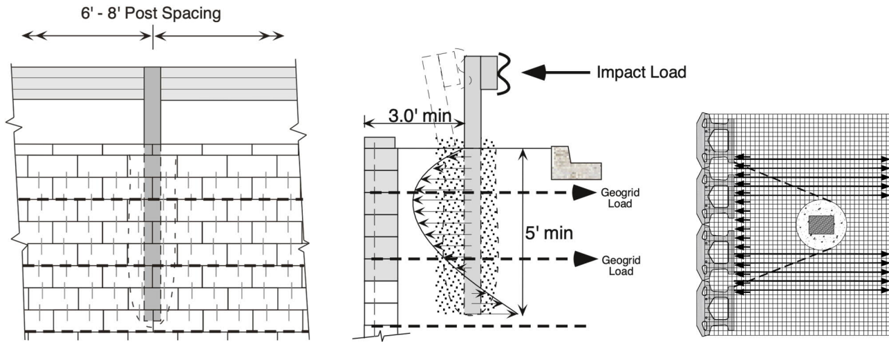
Typical Guiderail Elevation
